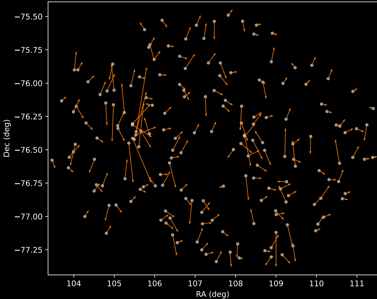
GALAH DR4 Cluster 2 Proper Motion Vectors (n=180)
