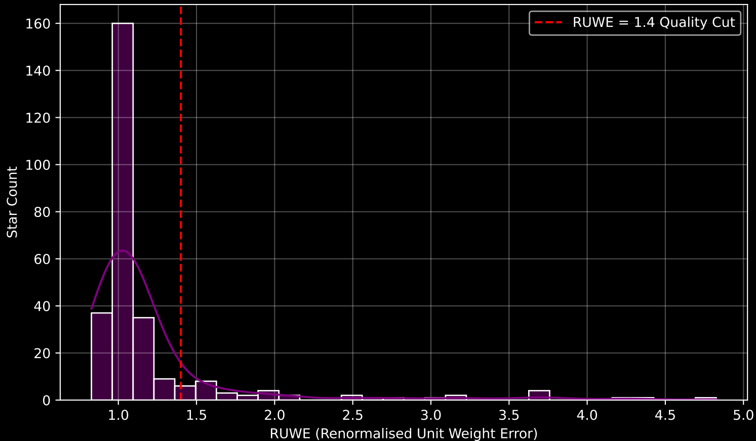
GALAH DR4 Field [181] RUWE Distribution (n= 280)
