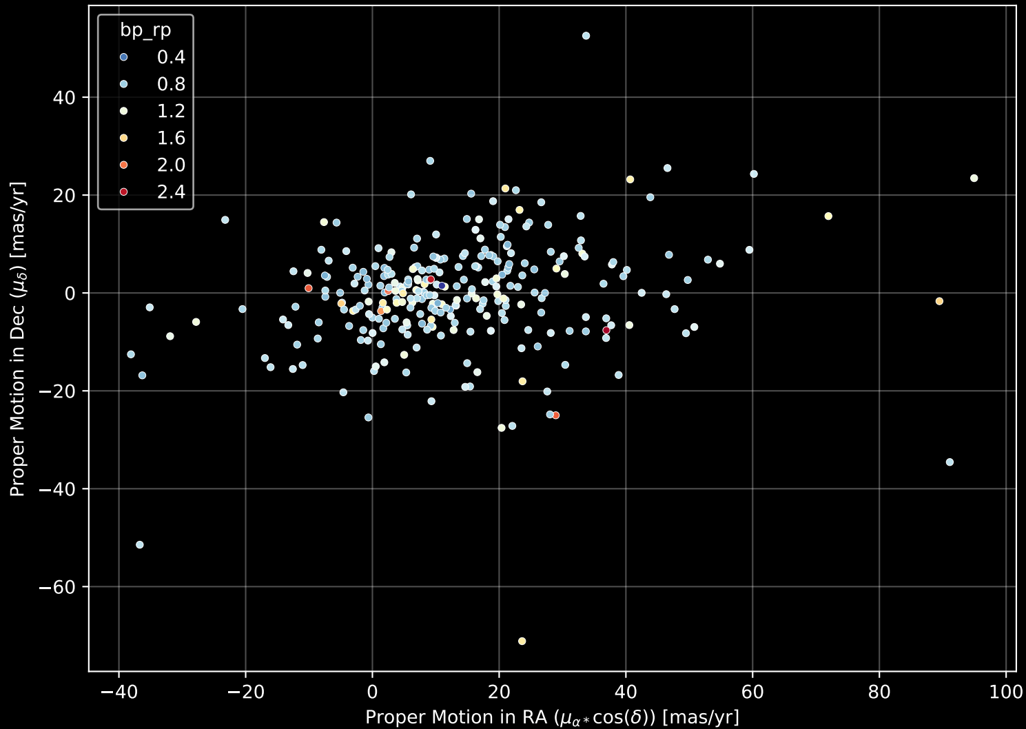
GALAH DR4 Field: [181] Proper Motion Diagram (n= 289)
